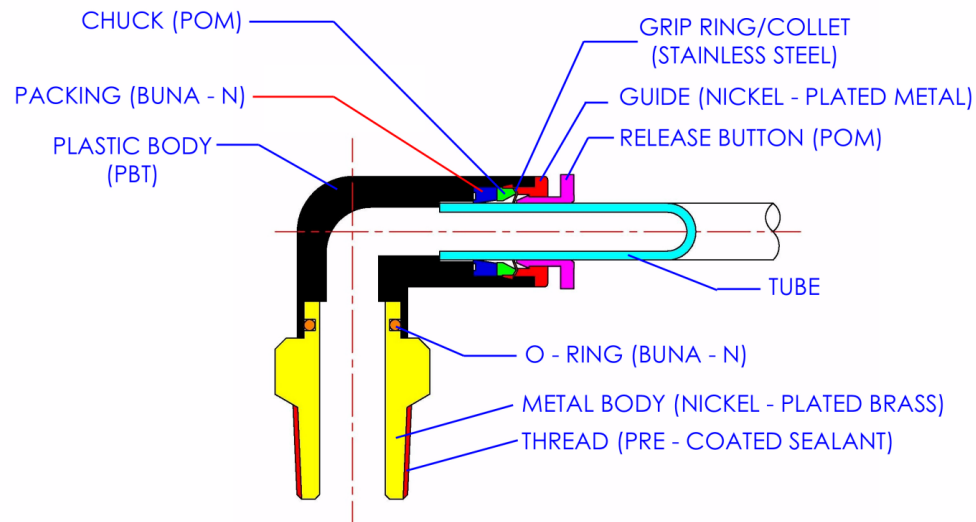
SCHEMATIC OF TYPICAL COMPOSITE FITTING CONSTRUCTION
